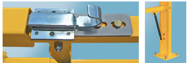
Safety Lock Mechanism, and Gas Struts for ease of operation
